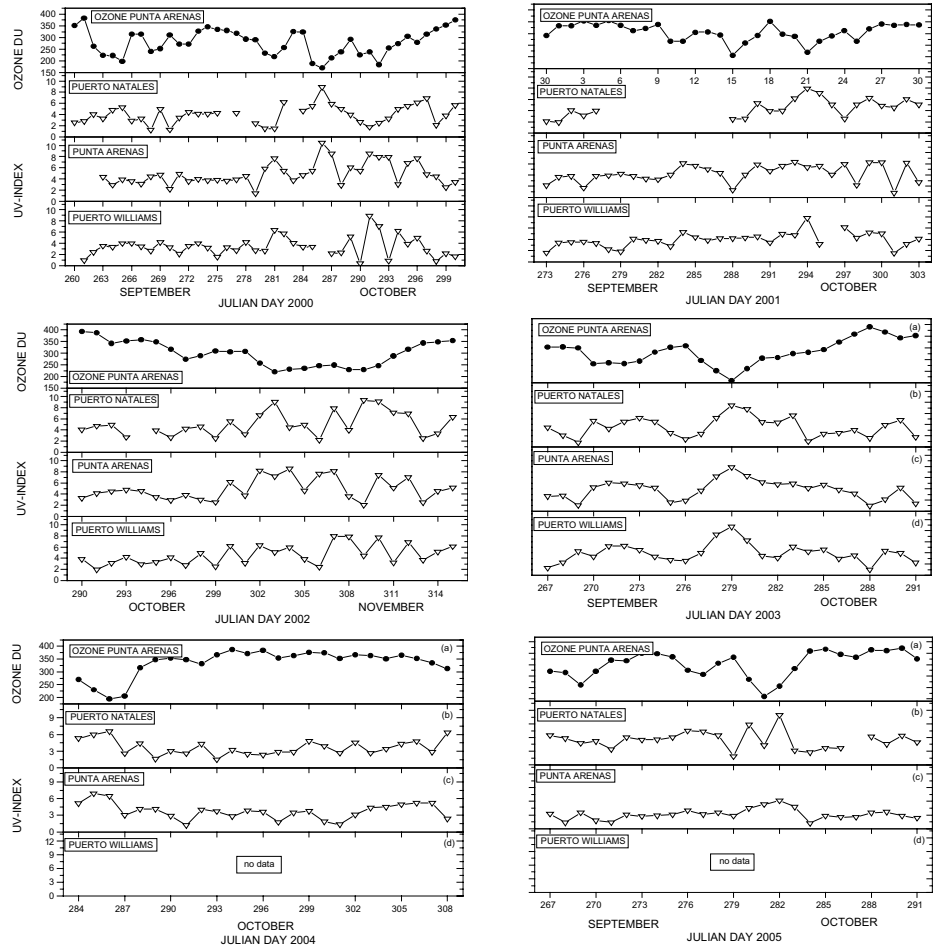
Fig. 6. UV-Index at the minimum solar angle during periods of the activity of the AOH over the Magallanes region. Ozone column measured at Punta Arenas is included.
